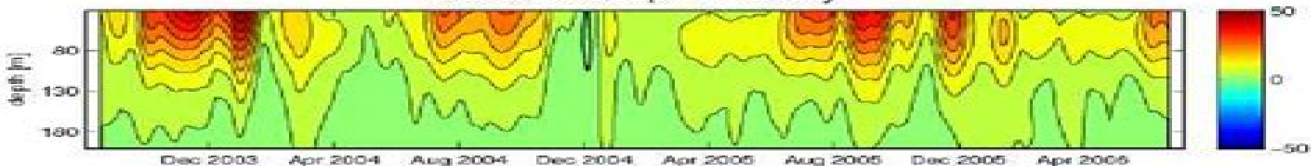
KS10 Geostrophic Velocity
